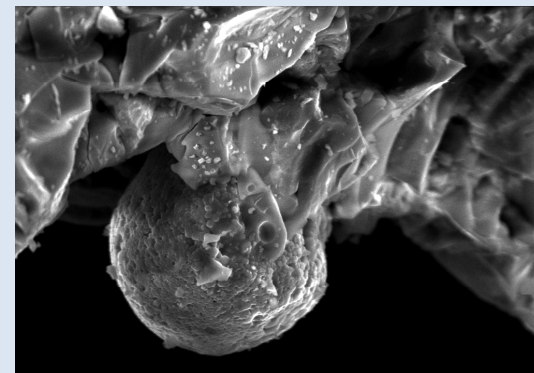
Wear debris in a ceramic nanocoating
